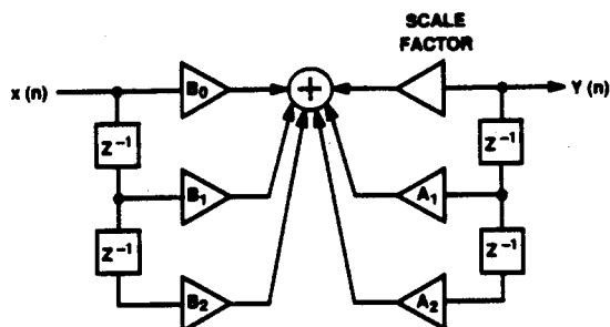
Figure 1. Second-Order Biquad IIR Filter Section
